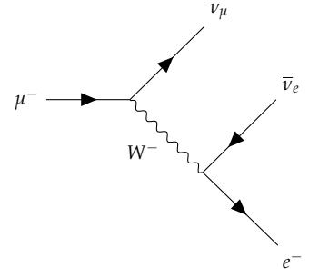
Figure 2.10: A Feynman diagram, which is read left-to-right rather than bottom-to-top.
