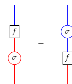
Figure 2.6: A morphism commuting with antipodes.
