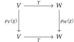
Figure 3.1: Commutative diagram for the intertwiner condition.
