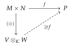
Figure 1.10: The universal property of the tensor product V \otimes_{\mathcal{K}} W .
